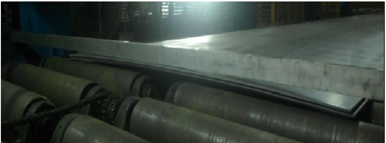
Figure 3 - Cross bow in hot-rolled steel plates or sheets and its measurement
