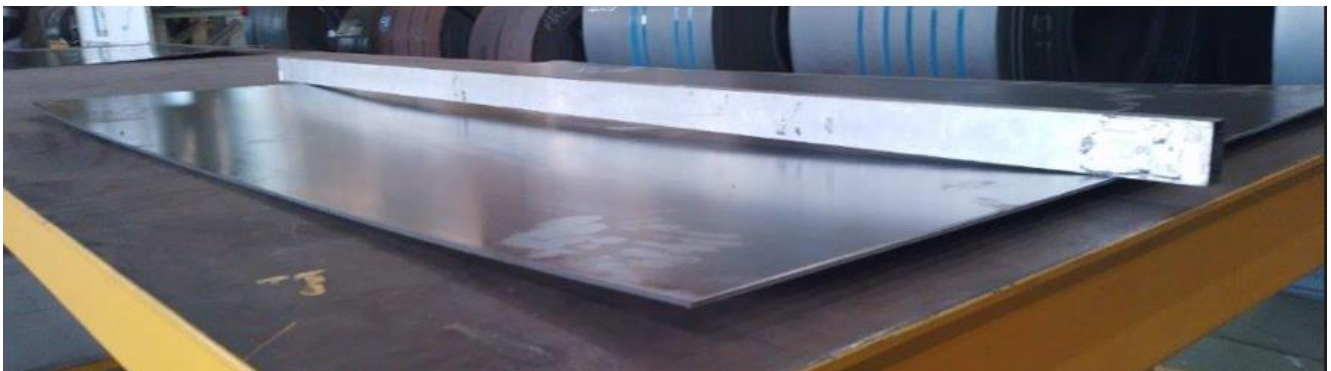
Figure 4 - Coil set in hot-rolled steel plates or sheets and its measurement
