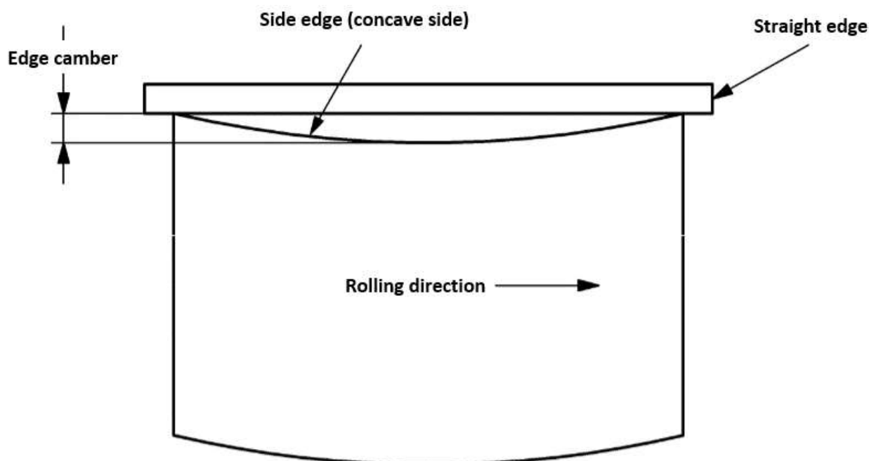
Figure 7 - Schematic drawing of steel plates and sheets edge camber measurement
