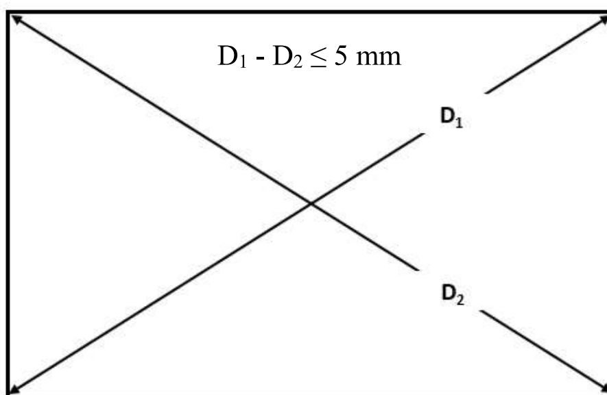
Figure 8 - Schematic drawing of steel plates and sheets out-of-squareness measurement
